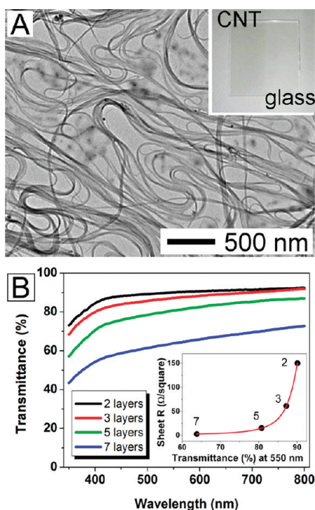
Figure 14. (A) TEM image of the single-layer SWCNT film made from IPA suspension. The inset shows the SWCNT film transferred on glass. (B) Transmittance characteristics of the multilayered SWCNT films made by multiple transfer of the SWCNT single layer to the PDMS substrate. Sheet resistance vs transmittance at 550 nm for each film is exhibited in the inset diagram.
