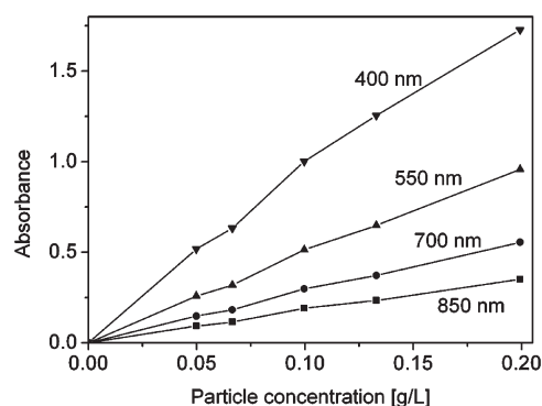
Figure 1. Standard curve showing the linear dependence of the PS particle concentration with absorbance, that is, light scattering, at different wavelengths.
